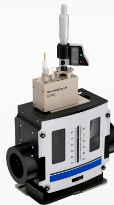
EC-IR2 Mounted on VeeMAX III
